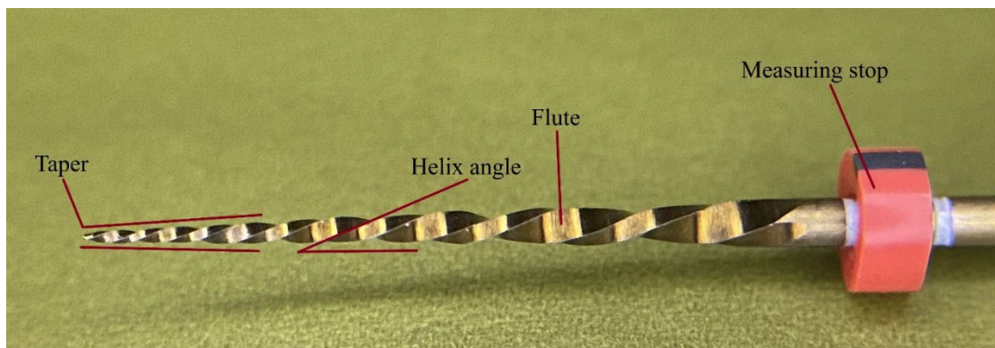
Figure 3: The WaveOne Gold file design
