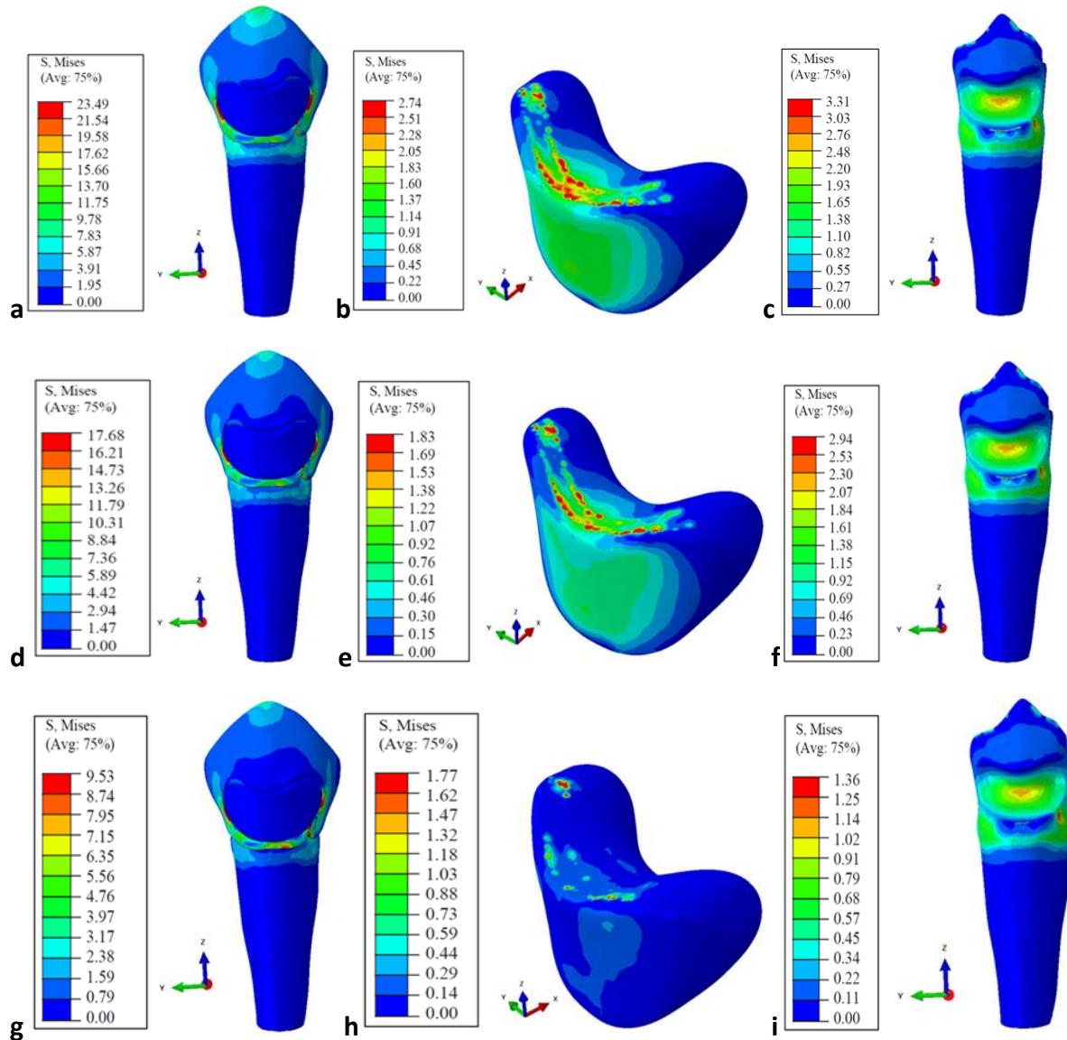
Figure 6a-l. Von Mises stress distributions during axial loading among different model components (enamel, dentin and restoration), with a-c corresponding to Model A; d-f, Model B; g-i, Model C; and j-l, Model D.
