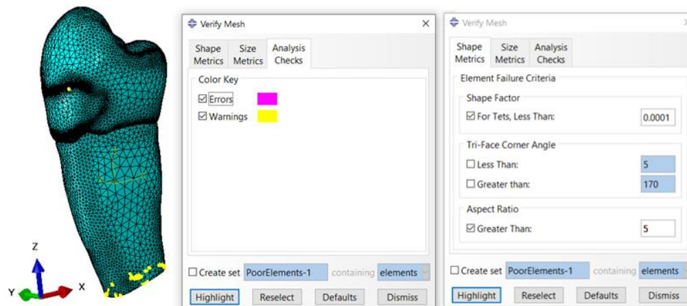
Figure 3. Mesh quality check of the 3D tooth model: The image shows mesh element warnings based on aspect ratio and shape quality to ensure accuracy and stability in the simulation.
