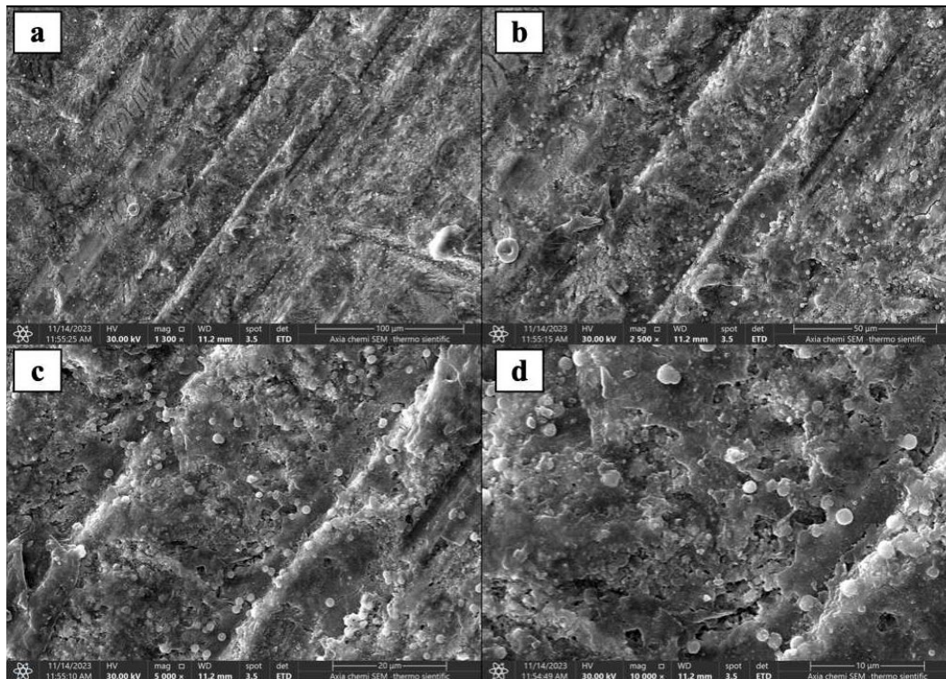
Figure 5: SEM for Group C zirconia specimen (Zircos-E treatment) at a) 1300x magnification, b) 2500x magnification, c) 5000x magnification, d) 10000x magnification.
