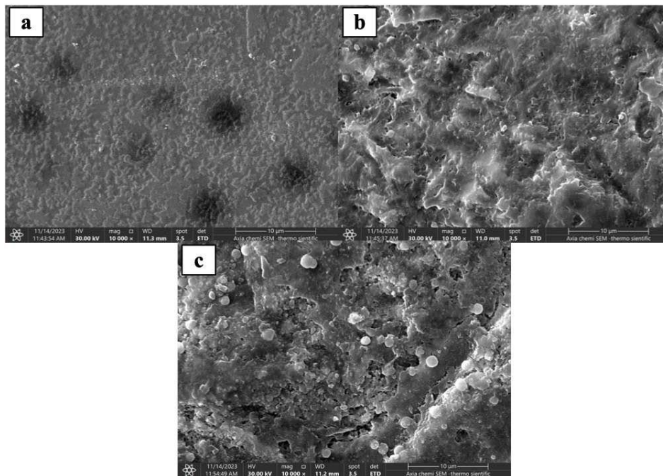
Figure 2: SEM at 10000x magnification a) Group A specimen (Un-treated zirconia), b) Group B zirconia specimen (airborne-particle abraded surface), c) Group D zirconia specimen (Zircos-E treatment).
