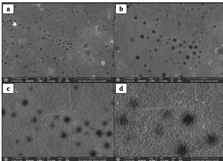
Figure 3: SEM for Group A zirconia specimen (Un-treated zirconia) at a) 1300x magnification, b) 2500x magnification, c) 5000x magnification, d) 10000x magnification.
