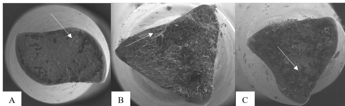
Figure 2: SEM fractographic analysis of fractured files tips (arrows pointing on the cracks lines); (A) fracture surface of EdgeOne Blaze Utopia file, (B) fracture surface of EdgeX7 Utopia file, (C) fracture surface of EdgeFile X7 file,
